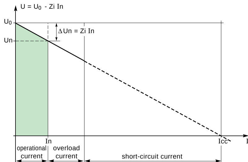
Fig. 1: incidence of internal impedance Z_i of energy sources on voltage delivered and their maximum short-circuit currents.
