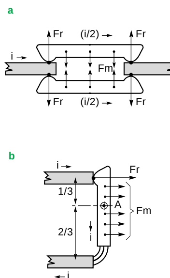
Fig. 24: reinforcement of contact electrodynamic withstand.
