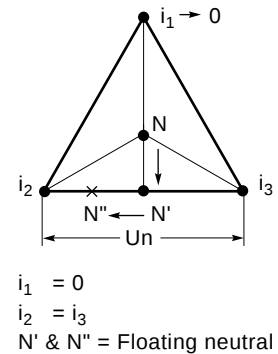
Fig. 12: with non-distributed neutral.
